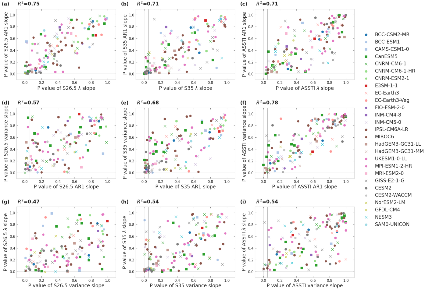
Figure E: Same as Fig 6 in the Main Text but for the correlations between the p-values of different CSD indicators.
