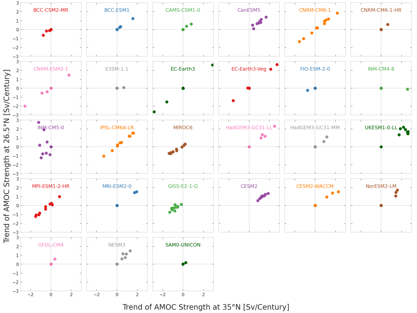
Figure A: For each model, the 1850–2014 trend in its ensemble members of the AMOC streamfunction strength at 26.5°N and at 35°N. Even though the aerosol forcing is the same within each model, there is still a large scatter of ensemble member slopes.
