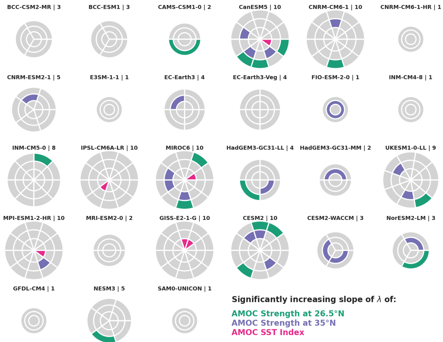
Figure I: Same as Fig 3 in the Main Text, but with a window size of 70 years.
