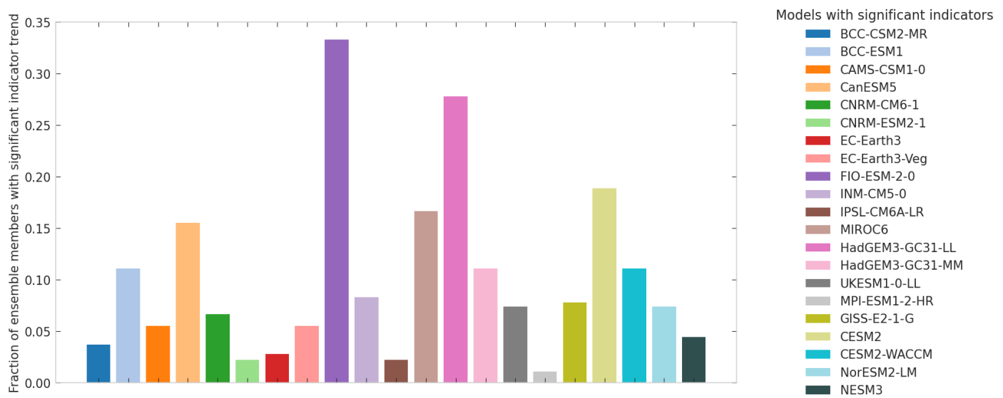
Figure D: Fraction of timeseries for a given model that have a significant increase in any of the three CSD indicators. Only the models that do have such significant increases are shown, and the full list of these can be found in Tables D, E, F in S1 Table. Note that the colours for the models are different from other figures.
