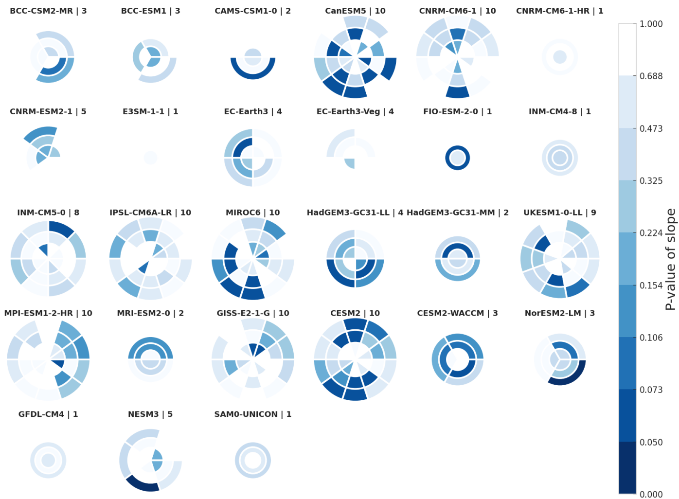
Figure C: Same as Fig 3 in the Main Text, but with the slices coloured according to the p-value of the corresponding \lambda . Darker blue is a smaller p-value and so more statistically significant.
