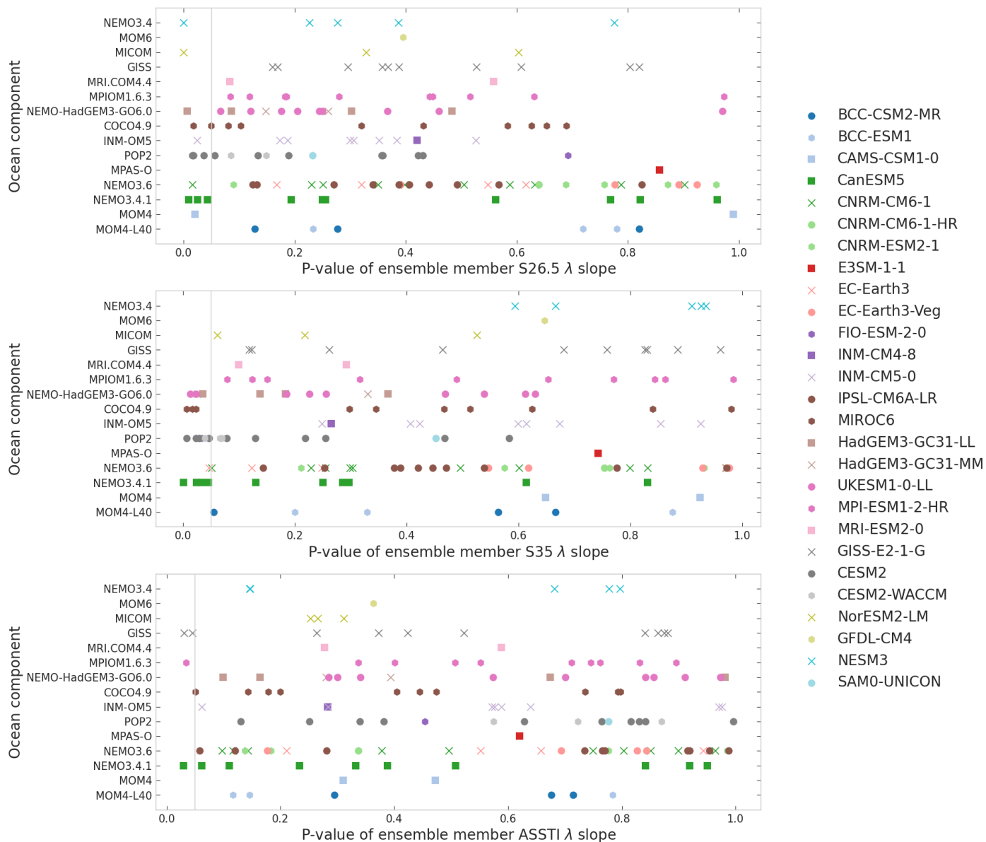
Figure M: The distribution of the ensemble member p-values for the \lambda trend of the AMOC streamfunction strengths at 26.5°N and 35°N and the AMOC SST Index, plotted against the ocean component of the model. The models with lower p-values have a range of different ocean components.
