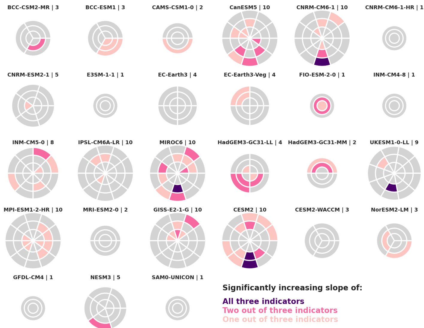
Figure J: Same as Fig 4 in the Main Text, but with a window size of 50 years.
