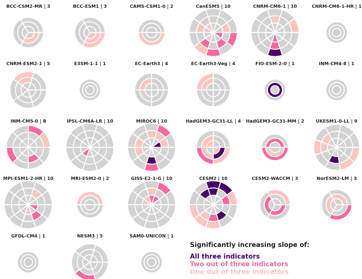
Figure K: Same as Fig 4 in the Main Text, but with a window size of 70 years.
