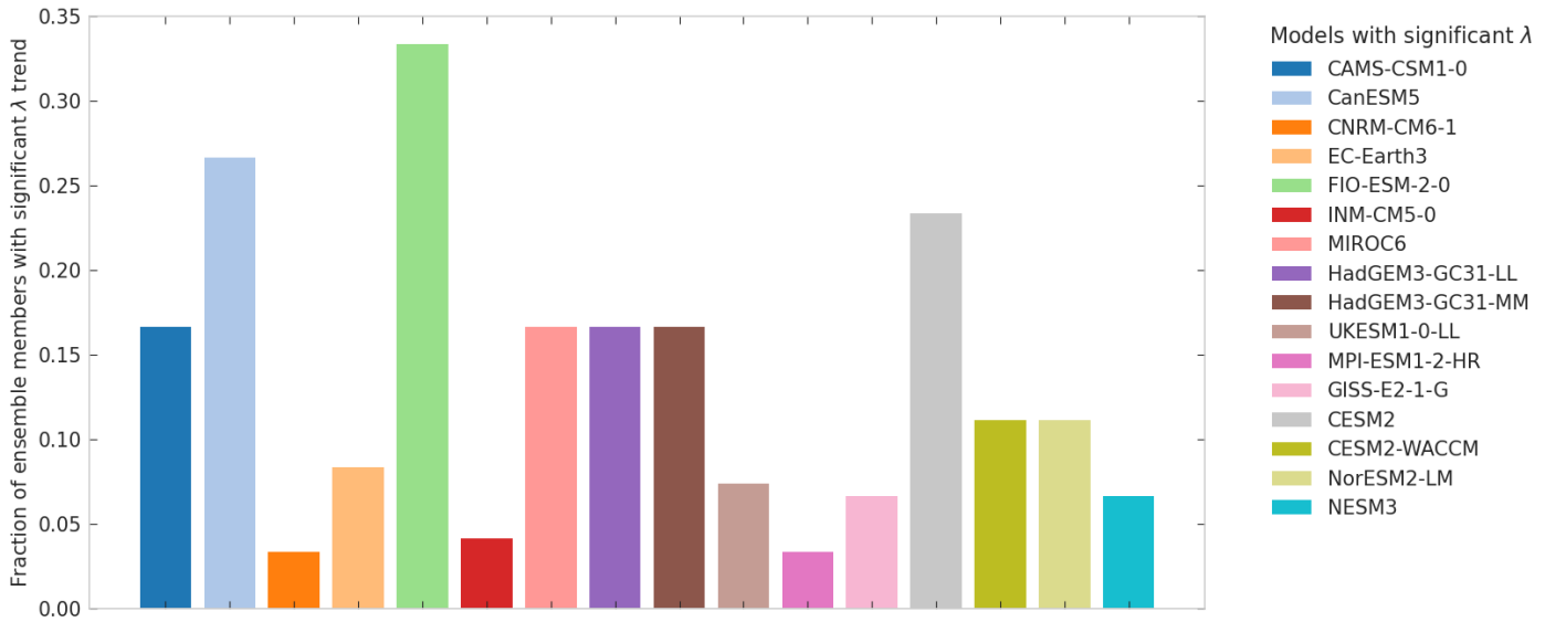
Figure B: Fraction of all timeseries for a given model that have a significant increase in \lambda (so both in streamfunction strength and SST Index). Only the models that do have such significant increases are shown, and the full list of these can be found in Table D in S1 Table. Note that the colours for the models are different from other figures.
