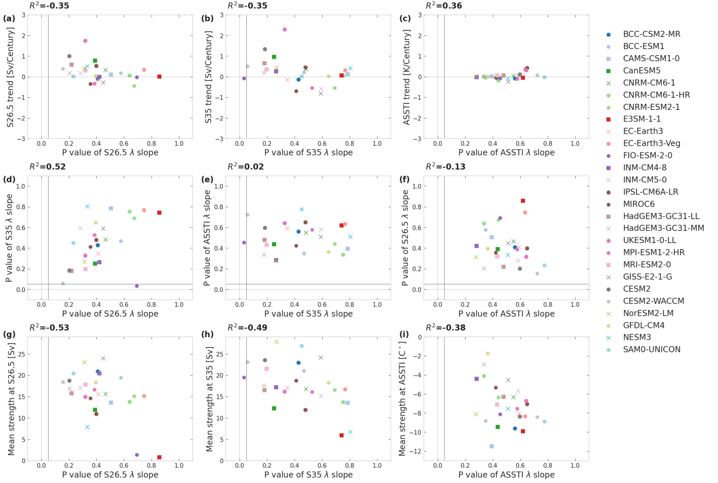
Figure L: Same as Fig 6 in the Main Text for the ensemble mean values of each of the models.
