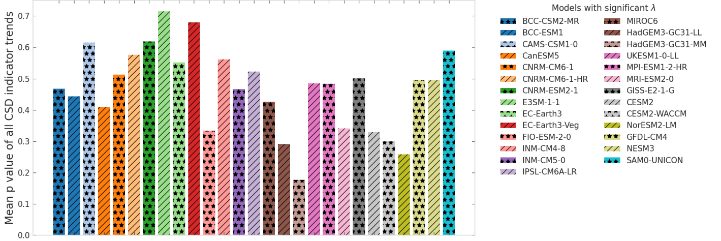
Figure O: Mean p-value for all CSD indicator timeseries of a given model. Note that the colours and shading of the models are different from other figures.
