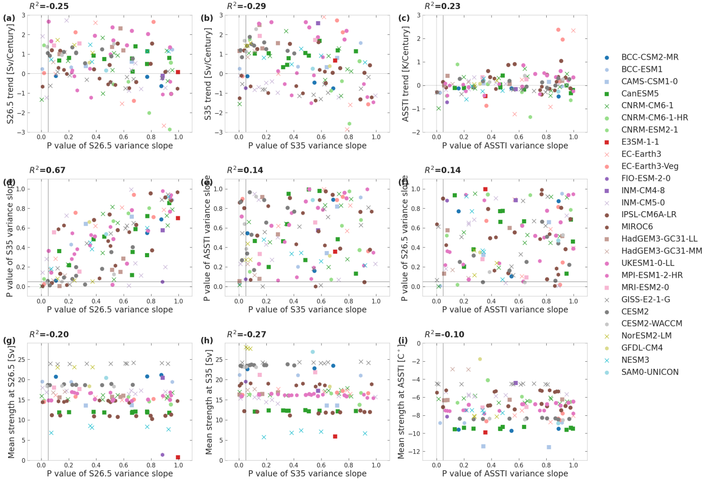
Figure G: Same as Fig 6 in the Main Text for the variance instead of \lambda .
