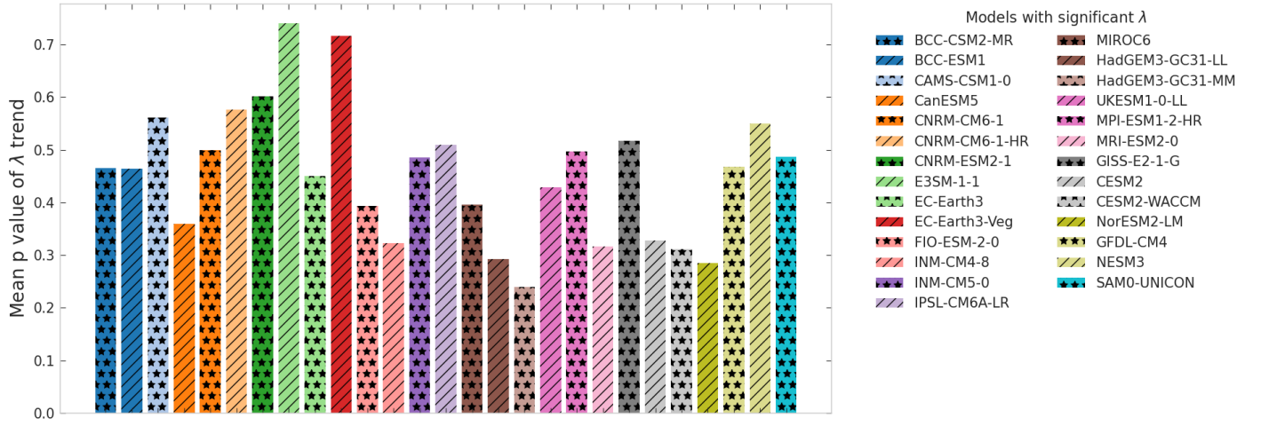
Figure N: Mean p-value for all \lambda timeseries of a given model. Note that the colours and shading of the models are different from other figures. Note that the models with highest indication of CSD are those with the lowest p-values.
