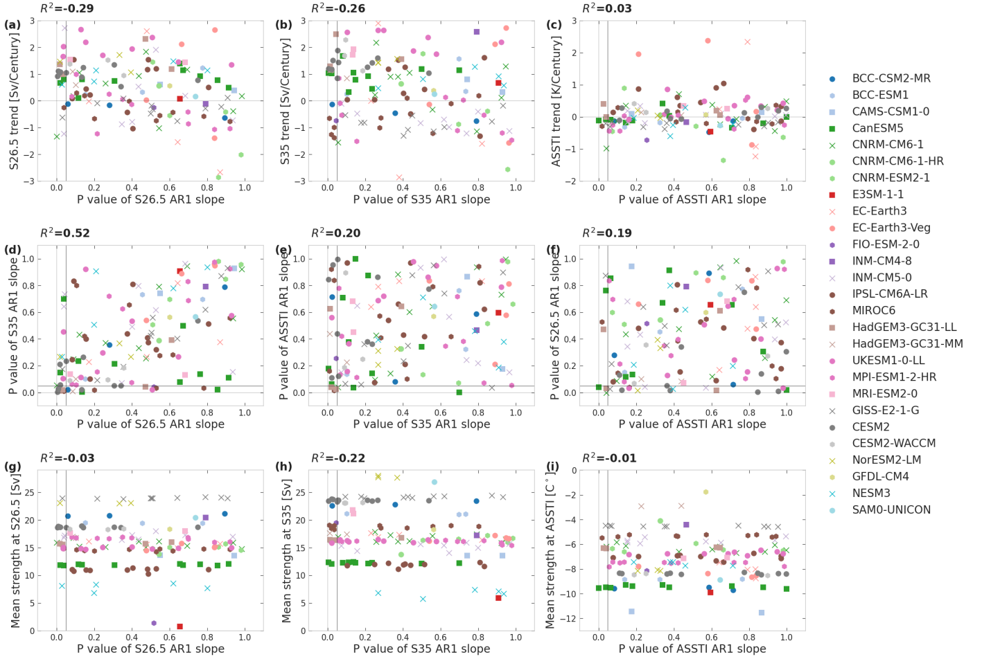
Figure F: Same as Fig 6 in the Main Text for the AR1 instead of \lambda .
