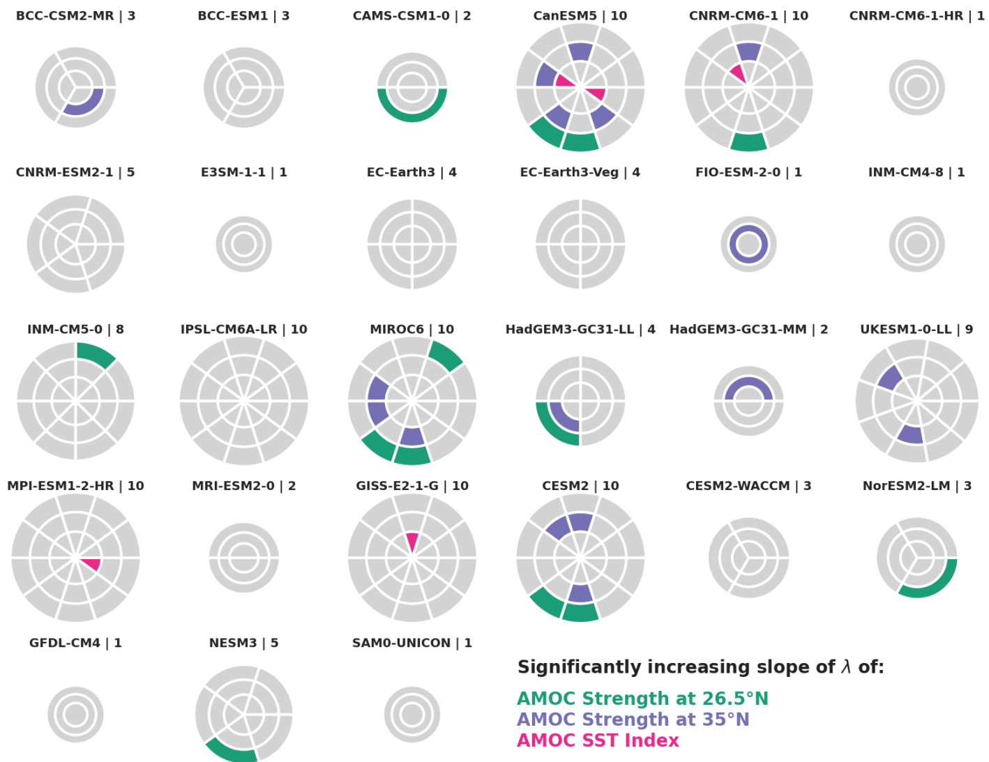
Figure H: Same as Fig 3 in the Main Text, but with a window size of 50 years.
